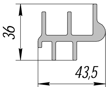
HP-589; 1,073кг/п.м.
