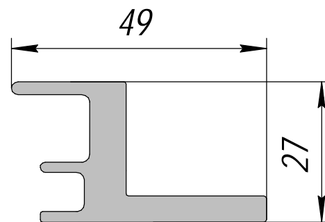
HP-508; 1,105кг/п.м.
