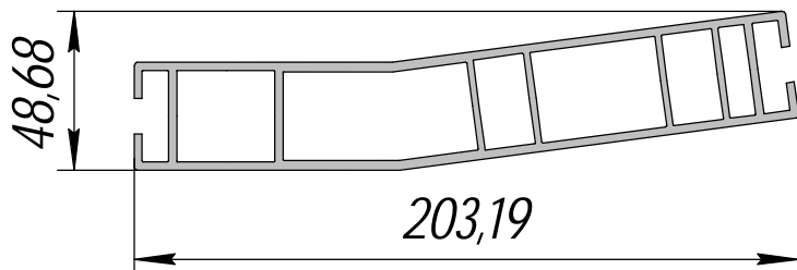
AC-81; 4,444кг2/п.м.
