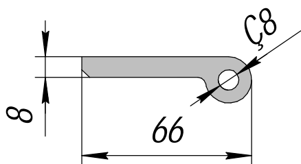
AC-85; 1,633кг2/п.м.
