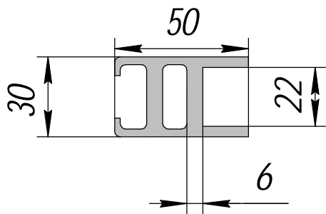
HP-436-01; 1,743кг/п.м.
