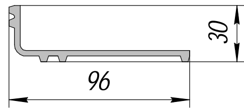
HP-376; 1,101кг/п.м.
