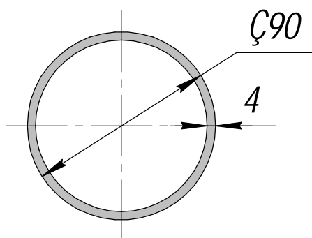
ПА-12; 2,929кг/п.м.
