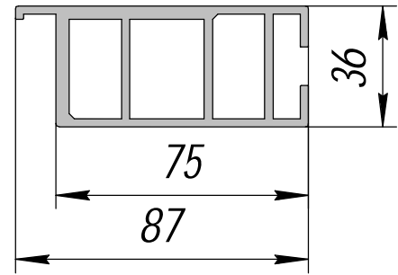
AC-75; 2,362кг/п.м.
