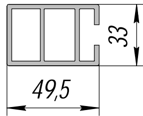
AC-78; 1,315кг/п.м.
