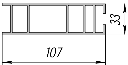
AC-81; 4,444кг2/п.м.
